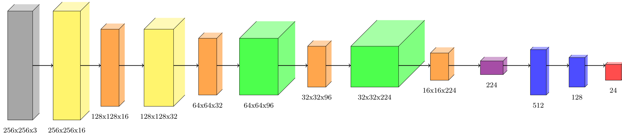
Figure 1 : Full CNN Architecture
